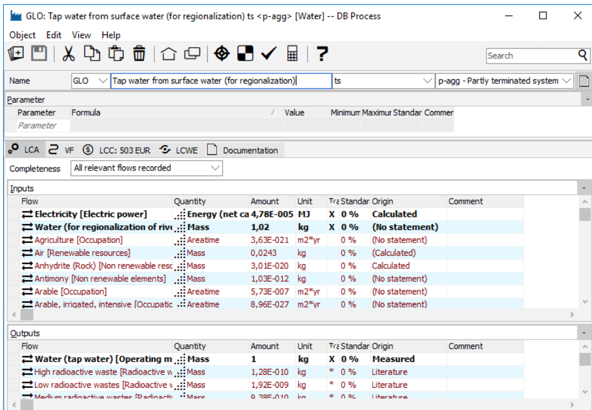
Figure 6: Provision of water (tap water) as partially aggregated process with open input flows
